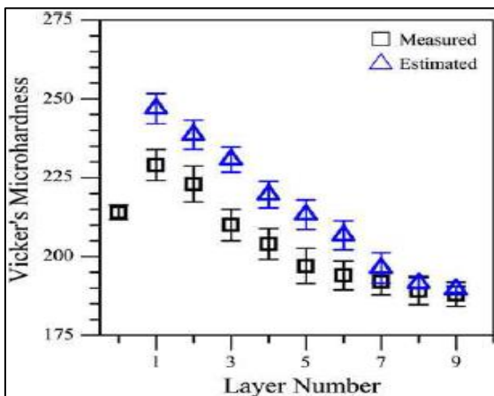
Fig 15: Comparison Between Estimated and Measured Micro-Hardness in Deposited Layers [9]
