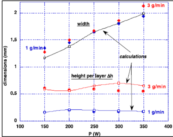
Fig 23: Comparison Between Experimental Data and Simulated Values, (a) Influence of Laser Power and Mass Feed Rate on the Stabilizing Geometrical Features of a DMD Wall [12]
