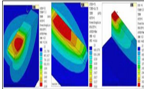
Fig 2: Same Power and Different Time Steps, (A) 2000W, 7.5s, (B) 2000W, 18.75s, (C) 2000W, 133.75s [2]
