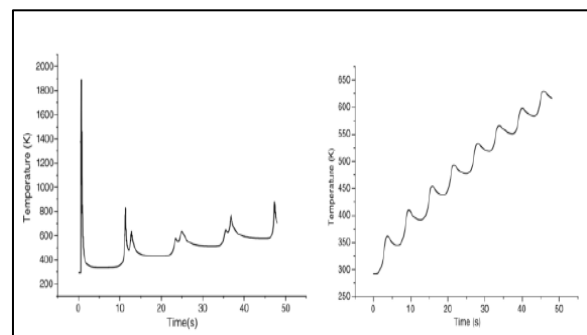
Fig 9: Thermal History of a Point in the Substrate (a) and in the Deposit (b) [4]
