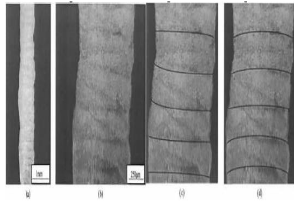
Fig 21: Comparison of Melt Pool Boundaries Obtained by the Processing Result of the Edge Detector with Those Obtained by the Modelling, (a) Original Image Acquired by High Shutter Speed Camera, (b) Processing Result of Edge Detector, (c) Numerical Modelling Result, (d) Analytical Modelling Result [11]
