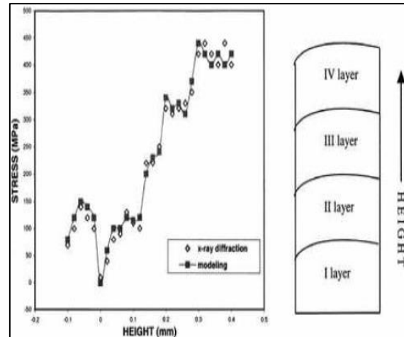
Fig 22: Distribution of Residual Stresses Within Subsequent Layer, Comparison Between X-Ray Diffraction Results and Modeling Results [11]
