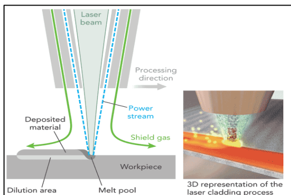
Fig 1: Schematic of LDMD Process[1].
