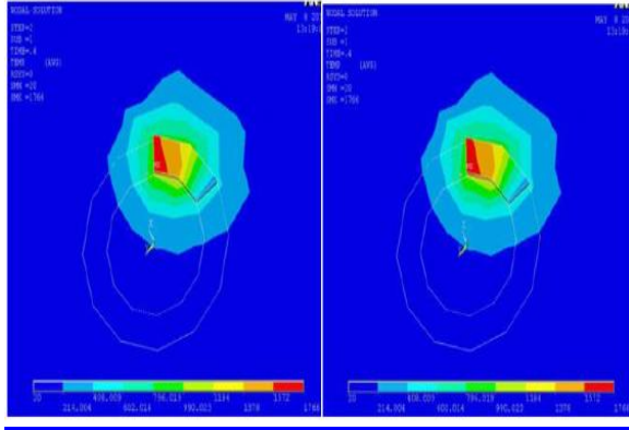
Fig 17: Temperature Field Distribution with Different Radius [10]
