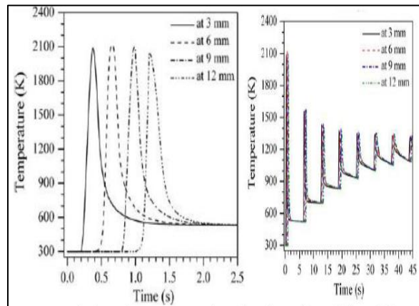
Fig 7: Variation of Temperature Along First Layer (a) and First Eight Layers (b) [3]
