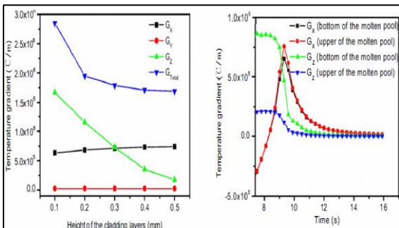
Fig 6: Variation of Temperature Gradient With Height and Time [2]
