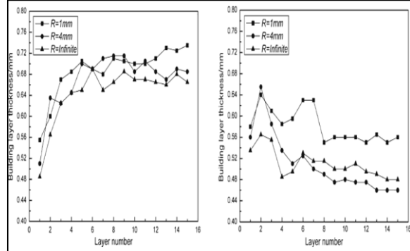
Fig 19: Relation Between Building Thickness and Layer Number, (a) with Constant Laser Power, (b) with Varied Laser Power [10]
