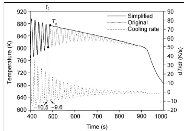
Fig 11: Sketch of the Simplification of Thermal History[7]
