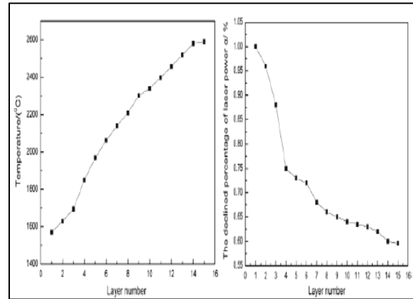
Fig 16: Relation Between Temperature Distribution and the Trend of Laser Power and Layer Number (a) Temperature Distribution (b) Trend of Laser Power Changing[10]
