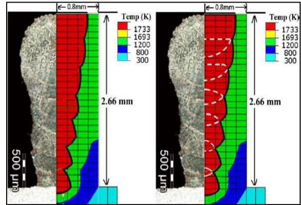
Fig 12: Actual and Simulated Melt Pool Profile [9]
