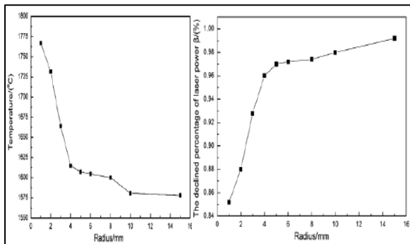
Fig 18: Relationship Between Temperature Distribution and Radius [10]
