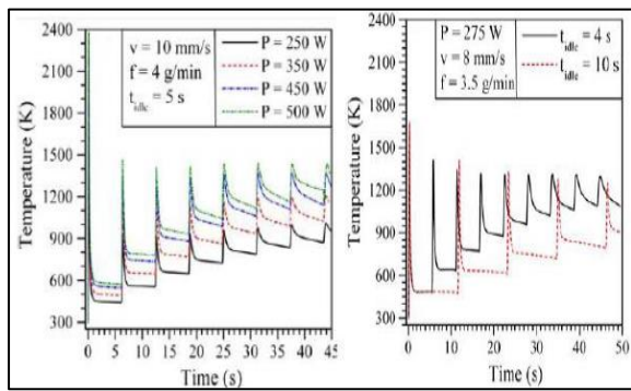
Fig 8: Variation of Temperature with Different Process Parameters [3]
