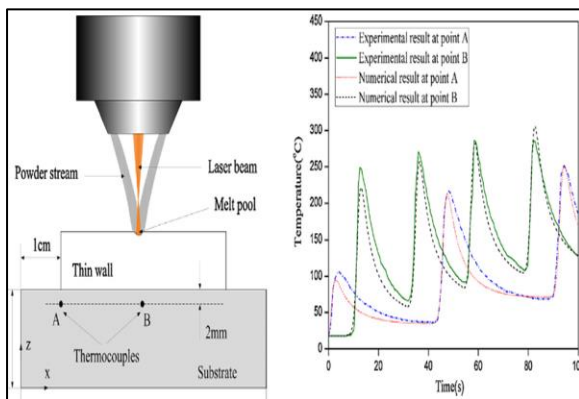
Fig 10: Comparison Between Simulated and Measured Values at Point a and B [5]
