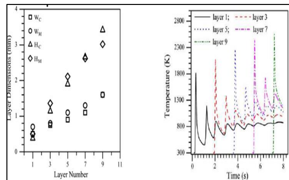
Fig 13: Computed and Measured Width and Height and Computed Thermal Cycles [9]
