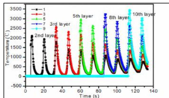
Fig. 3: Temperature Time History of Mid-Section [2]
