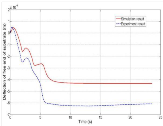
Fig 27: Simulation and Experimental Results of Deflection of Substrate [13]
